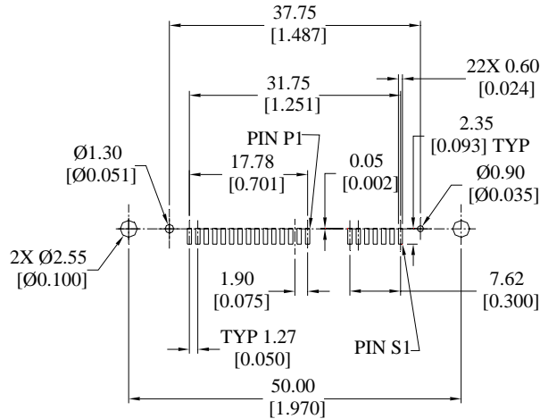
RECOMMENDED PCB LAYOUT TOLERANCE: ± 0.05 [0.002]
